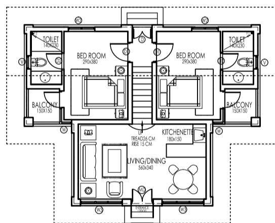
PLAN PLINTH AREA= 710 SQ.F
