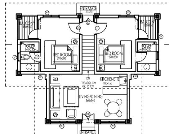
PLAN PLINTH AREA= 710 SQ.F
